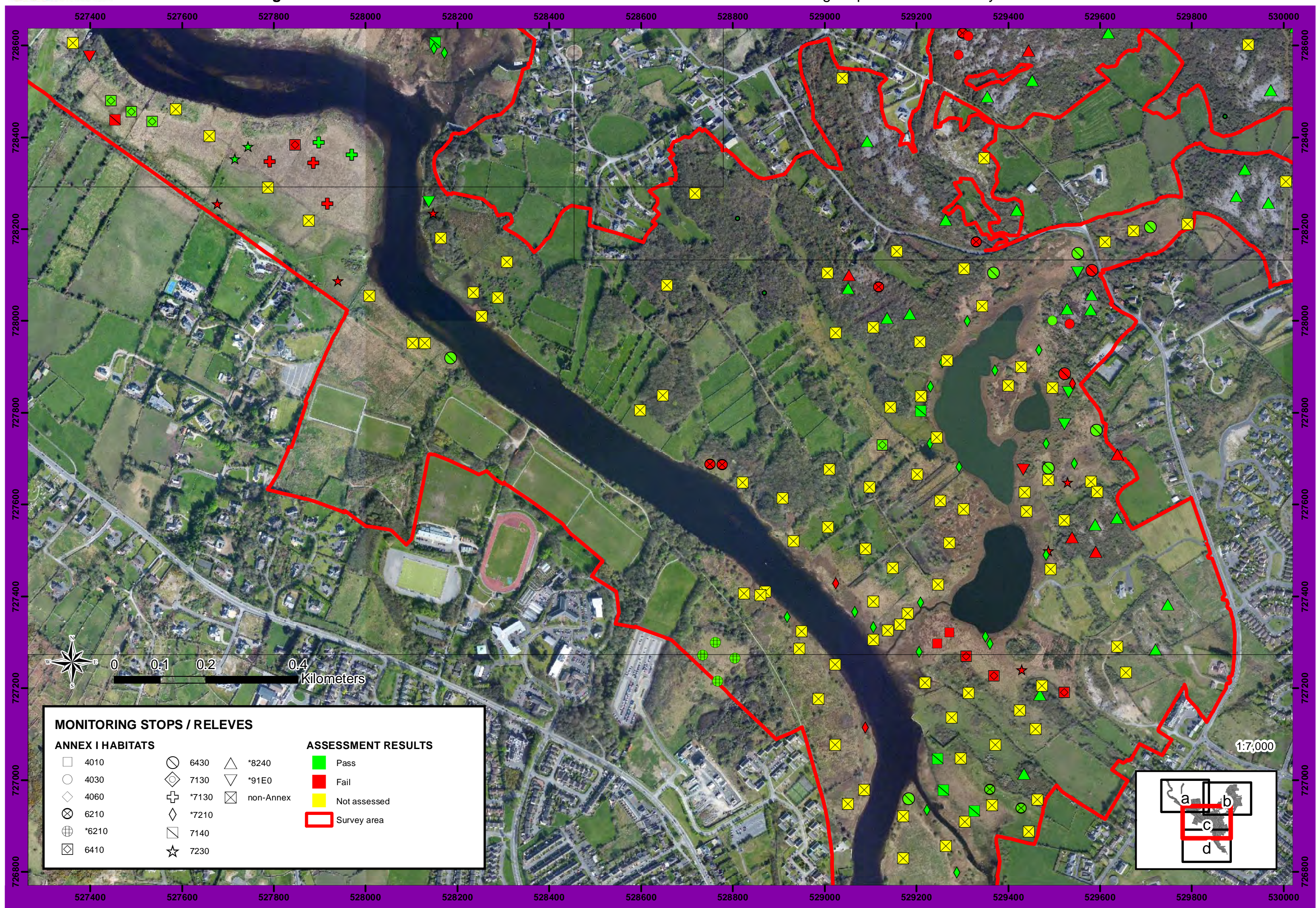
Figure 5c. Location of relevés and results of conservation assessment monitoring stops within the survey area
