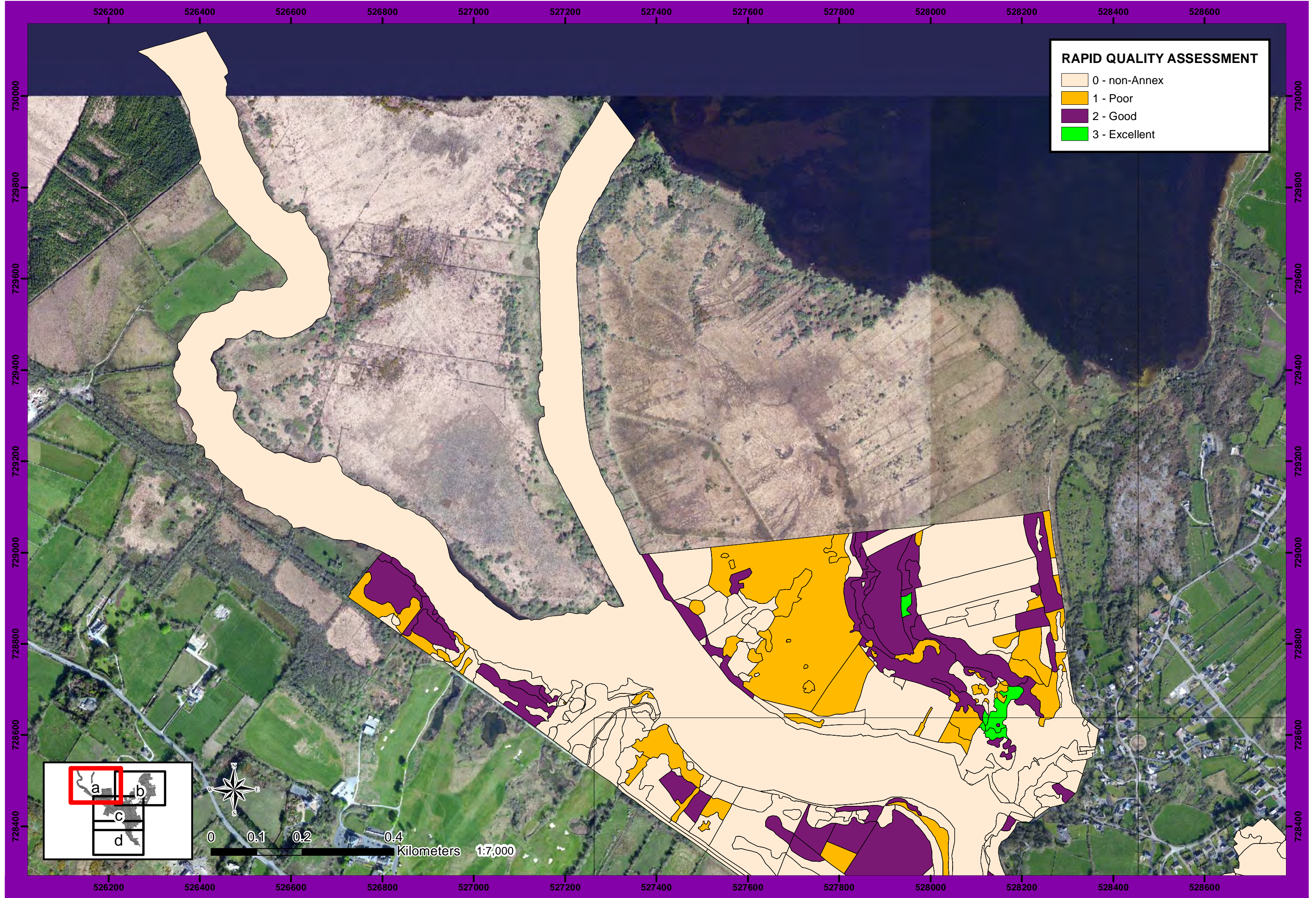
Figure 4a. Rapid assessment of Annex I habitat quality within the survey area
